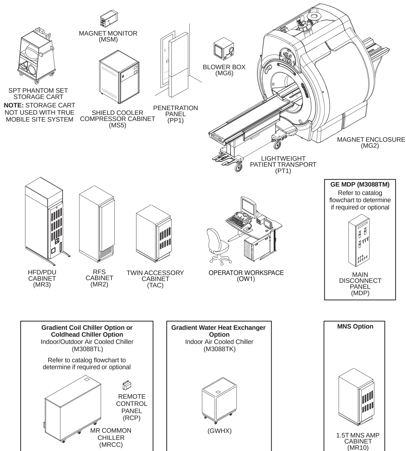
SIGNA EXCITE 1.5T SYSTEM ILLUSTRATION 1-1
